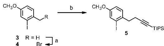
Scheme 1. Synthesis of the benzene building block 5 . Reagents and conditions: (a) NBS (1.1 equiv.), AIBN (cat.), K 2 CO 3 (cat.), CCl 4 , reflux, 1 h, 99%; (b) LiCH 2 C≡CTIPS (1.0 equiv.), THF, -78 °C, 10 min, 74%.
