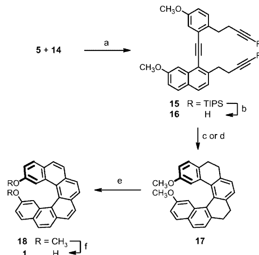
Scheme 3. Synthesis of 2,15-dihydroxyhexahelicene 1 . Reagents and conditions: (a) 5 (1.0 equiv.), 14 (1.0 equiv.), \text{Pd}(\text{PPh}_3)_4 (5%), \text{CuI} (10%), i\text{Pr}_2\text{NH} , 80^\circ\text{C} , 10 min, 79%; (b) n\text{Bu}_4\text{NF} (2.4 equiv.), THF, r.t., 1 h, 84%; (c) \text{CpCo}(\text{CO})_2 (20%), \text{PPh}_3 (40%), n -decane, halogen lamp, 140^\circ\text{C} , 1 h, 56%; (d) \text{Ni}(\text{cod})_2 (20%), \text{PPh}_3 (40%), THF, r.t., 24 h, 53%; (e) \text{Ph}_3\text{CBF}_4 (3.0 equiv.), 1,2-dichloroethane, 85^\circ\text{C} , 12 h, 64%; (f) \text{BBr}_3 (10 equiv.), \text{CH}_2\text{Cl}_2 , 0^\circ\text{C} to r.t., 2 h, 52%.
