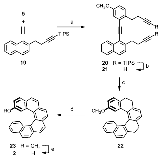
Scheme 4. Synthesis of 2-hydroxyhexahelicene 2 . Reagents and conditions: (a) 5 (1.0 equiv.), 19 (1.0 equiv.), \text{Pd}(\text{PPh}_3)_4 (2.5%), \text{CuI} (5%), i\text{Pr}_2\text{NH} , 80^\circ\text{C} , 10 min, 86%; (b) n\text{Bu}_4\text{NF} (2.4 equiv.), THF, r.t., 1 h, 60%; (c) \text{CpCo}(\text{CO})_2 (20%), \text{PPh}_3 (40%), n -decane, halogen lamp, 140^\circ\text{C} , 3 h, 77%; (d) \text{Ph}_3\text{CBF}_4 (3.0 equiv.), 1,2-dichloroethane, 80^\circ\text{C} , 3 h, 96%; (e) \text{BBr}_3 (4.5 equiv.), \text{CH}_2\text{Cl}_2 , r.t., 1 h, 95%.
