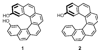
Figure 1. 2-Hydroxy- and 2,15-dihydroxyhexahelicene.
