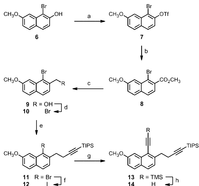
Scheme 2. Synthesis of the naphthalene building block 14 . Reagents and conditions: (a) n\text{BuLi} (1.0 equiv.), THF, -78^\circ\text{C} , 5 min, then \text{TiF}_2\text{O} (1.3 equiv.), -78^\circ\text{C} , 40 min, 67%; (b) \text{CO} , \text{Pd}(\text{OAc})_2 (5%), \text{dppp} (5%), \text{Et}_3\text{N} (2.5 equiv.), \text{DMSO}/\text{CH}_3\text{OH} , 3:2, 70^\circ\text{C} , 2 h, 58%; (c) \text{LiAlH}_4 (0.6 equiv.), THF, 0^\circ\text{C} , 1 h, 90%; (d) \text{PBr}_3 (1.3 equiv.), THF, 0^\circ\text{C} , 2.5 h, 67%; (e) \text{LiCH}_2\text{C}\equiv\text{CTIPS} (1.0 equiv.), THF, -78^\circ\text{C} , 1 h, 77%; (f) n\text{BuLi} (1.1 equiv.), THF, -78^\circ\text{C} , 10 min, then \text{I}_2 (1.5 equiv.), -78^\circ\text{C} , 20 min, 95%; (g) \text{TMSC}\equiv\text{CH} (1.6 equiv.), \text{Pd}(\text{PPh}_3)_4 (5%), \text{CuI} (10%), i\text{Pr}_2\text{NH} , in a sealed tube, 80^\circ\text{C} , 1 h, 99%; (h) \text{CH}_3\text{ONa} (2.4 equiv.), \text{CH}_3\text{OH} , r.t., 2 h, 99%.
